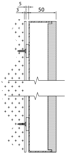
WALL FIXING
