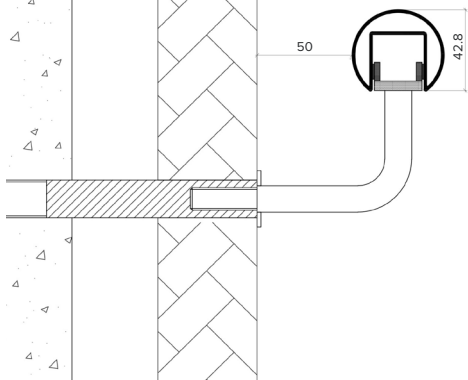
Wall Bracket
