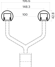
Asymetric Post Bracket
